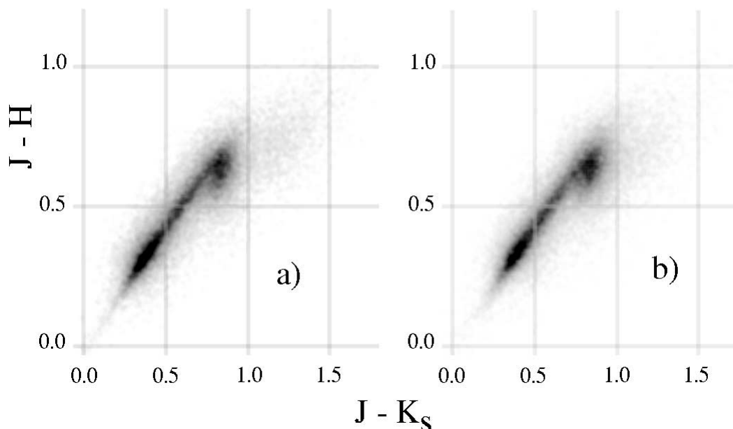
FIG. 19.—Hess diagrams of color-color distributions obtained for two different regions of the sky: (a) a “local” region of northern hemisphere data from the night of 1999 February 28 UT (about 30 deg 2 ); (b) sources randomly selected from Galactic latitudes below b = -40^\circ and between declinations -40^\circ and -70^\circ in the southern hemisphere, thus including data from hundreds of nights. The similarity of the distributions confirms the consistency of the nightly calibration solutions. The differences in the faint distribution of sources for J - K_s > 1.0 reflects actual differences in extragalactic populations in the “local” vs. “global” samples.
