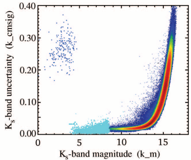
FIG. 17.—Reported default uncertainty ( k\_cmsig ) as a function of magnitude for the K_s band. Faintward of K_s \sim 9 a Hess diagram represents the density of occurrence of different values of k\_cmsig in the Point Source Catalog. For 4 < K_s < 9 , light blue points represent the uncertainties for individual sources that were saturated in the 1.3 s standard exposure time but were unsaturated in the 51 ms exposures. The dark blue individual points for K_s < 4 represent the uncertainties for sources that saturated the 51 ms exposures whose fluxes were estimated from fits to the unsaturated wings of the stellar profile.
