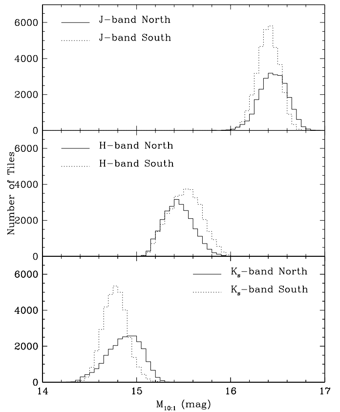
FIG. 16.—Histograms of the distribution of the S/N = 10 sensitivity level divided by hemisphere for each of the 59,731 scans that comprise the 2MASS catalogs.
