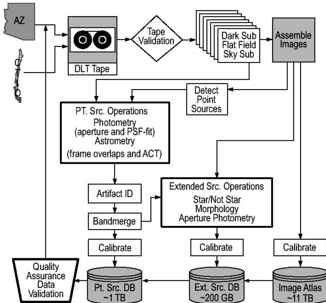
FIG. 12.—2MAPPS flowchart.
