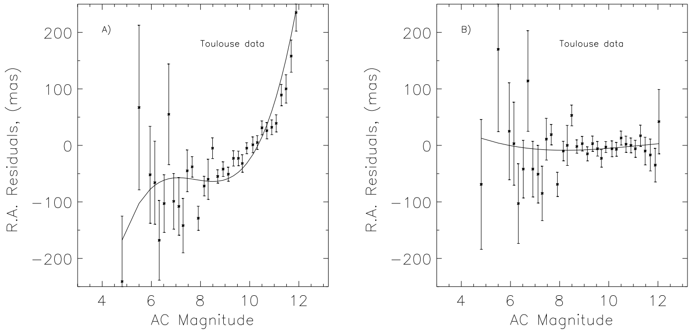
FIG. 4.—Differences in right ascension between the Toulouse zone and Hipparcos data as a function of magnitude, both (a) prior to the application of corrections and (b) following the corrections. Curves represent a third-order least-squares fit to the data points. Each point is the average of all stars in a 0.2 magnitude range.
