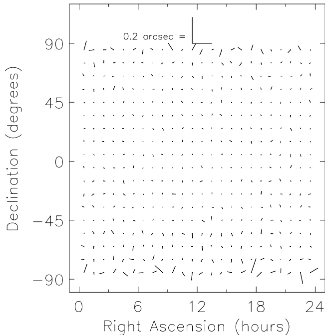
FIG. 5.—Systematic differences between the AC 2000 and Hipparcos , at the AC epoch. The data have not been smoothed. Each point is an average residual within a 1^h \times 10^\circ area. Near the poles few stars are contained within each area, and the random errors dominate. The standard deviation of each “point” spans from 11 mas per coordinate in the equatorial regions to 35 mas per coordinate at the poles. The lack of any noticeable pattern such as those seen in Fig. 3 demonstrates that the conversion to the Hipparcos system was successful. Note the scale difference between Fig. 3 and this plot.
