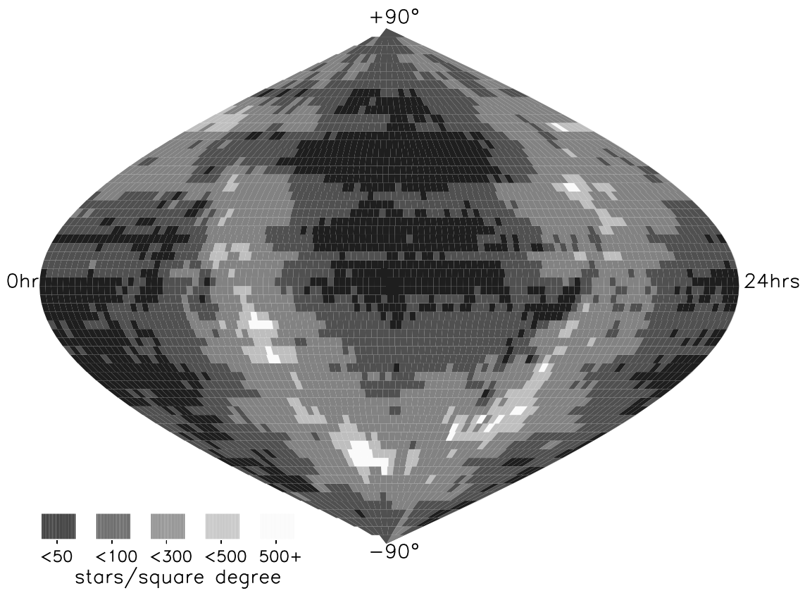
FIG. 8.—Stellar density of AC 2000
