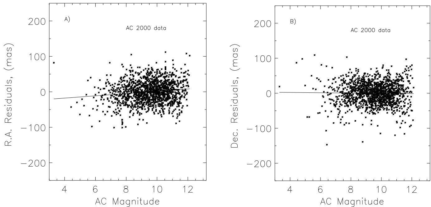
FIG. 6.—Positional differences between AC 2000 and Hipparcos by magnitude. For clarity, error bars are omitted, but are typically \pm 30 mas in size. Each point is the average of 200 observations.
