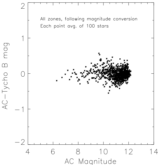
FIG. 2.—Differences in magnitude between the AC data and Tycho B data following conversion to the Tycho system. Each point is the average of 100 stars. For clarity, only every 25th point is plotted.
