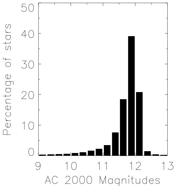
FIG. 11.—Magnitude distribution of AC 2000
