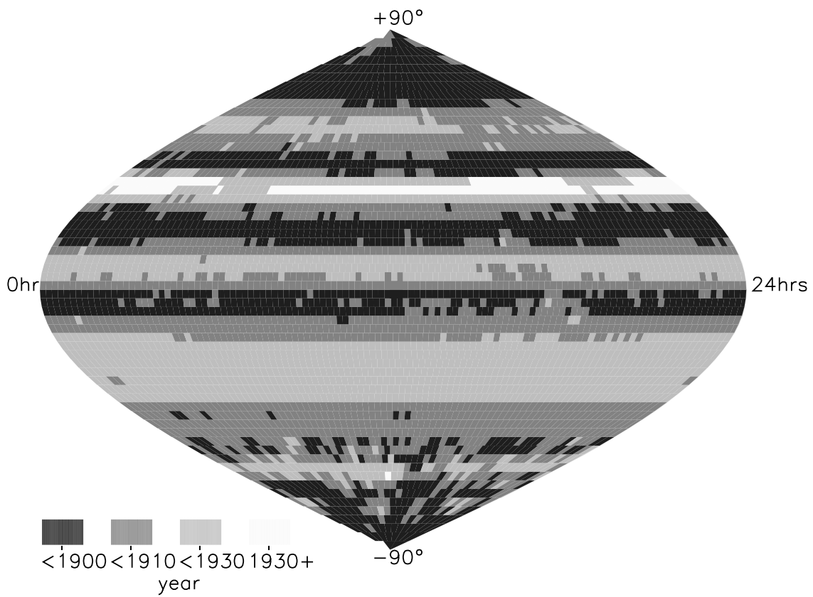
FIG. 9.—Mean epochs of AC 2000
