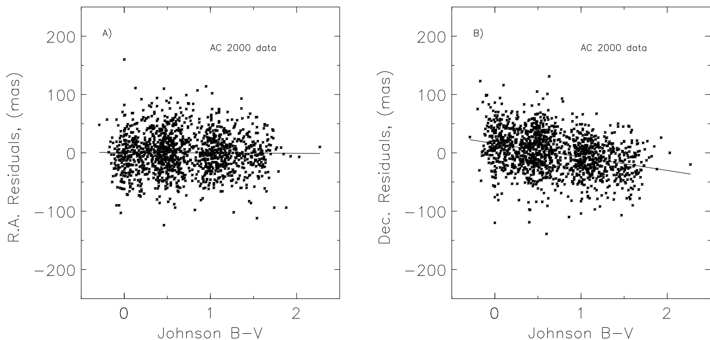
FIG. 7.—Same as Fig. 6, but by color index
