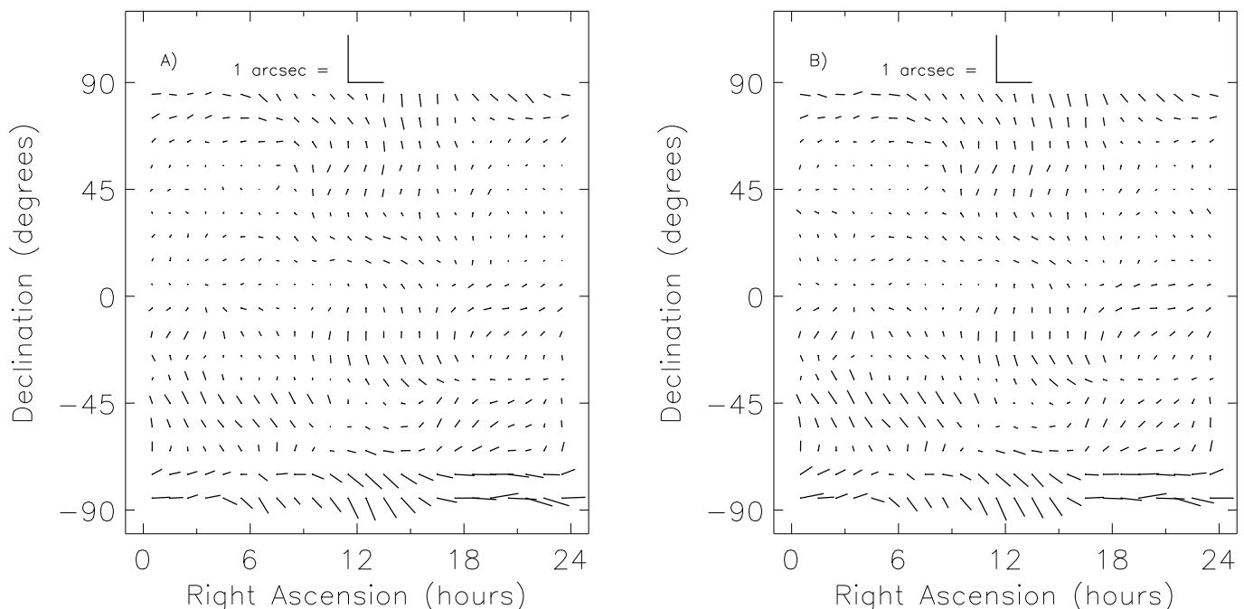
FIG. 3.—(a) Systematic differences between the AC/FK5 and Hipparcos . (b) Differences between ACRS at epoch 1900.0 and Hipparcos . The data have been lightly smoothed (that is, some effect from adjacent bins is present) to minimize random noise. The similarity of the two plots demonstrates that the AC/FK5 is indeed on the system defined by the ACRS, but a further reduction to the Hipparcos system is required.
